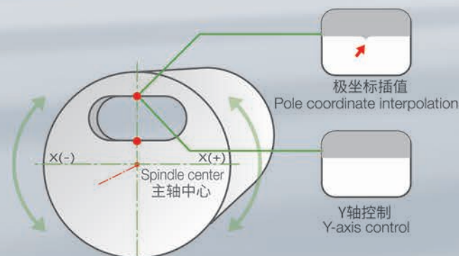
极坐标插值V.S Y轴控制 Pole coordinate interpolation V.S Y-axis control
